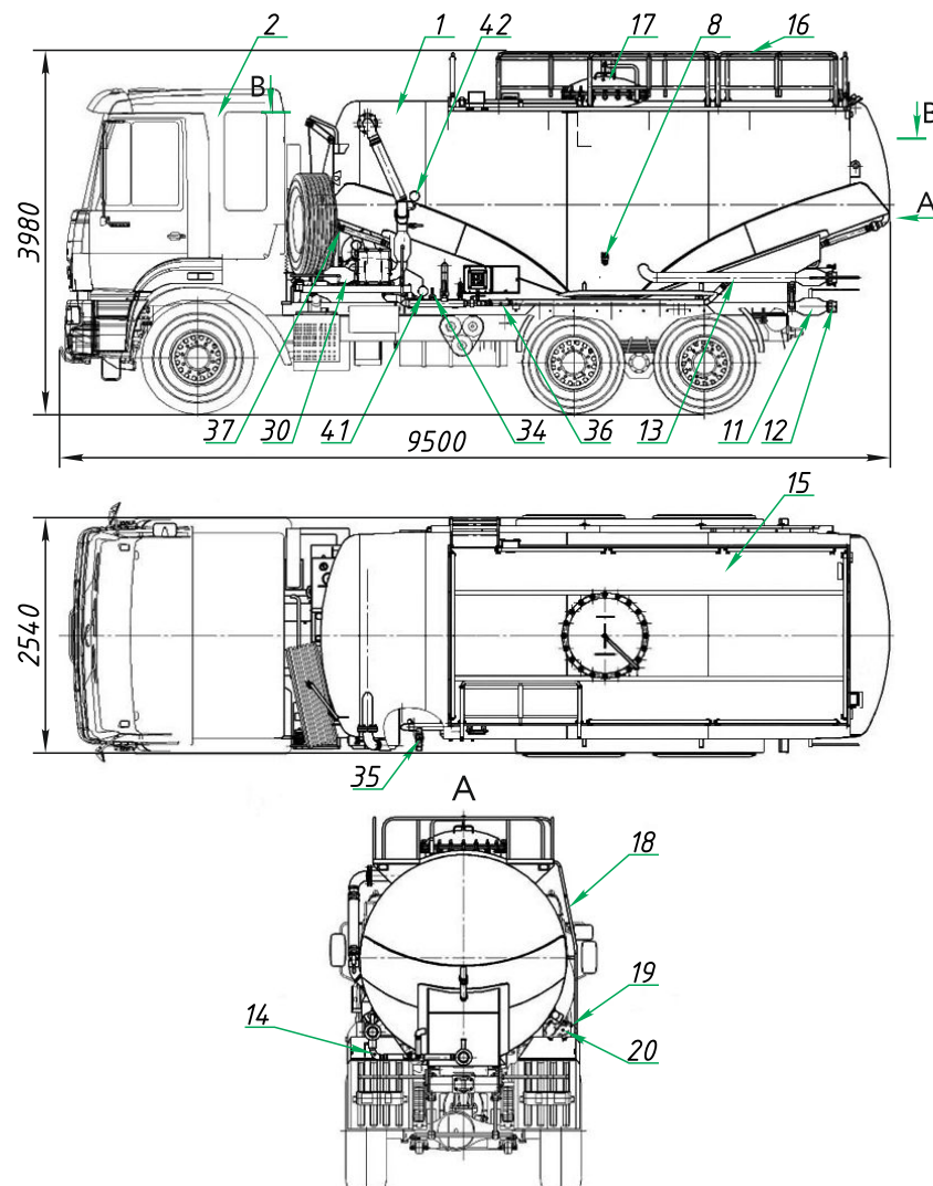
Figure 2 - ACV-17R1-09 Cement bulk truck. Structure and dimensions.
