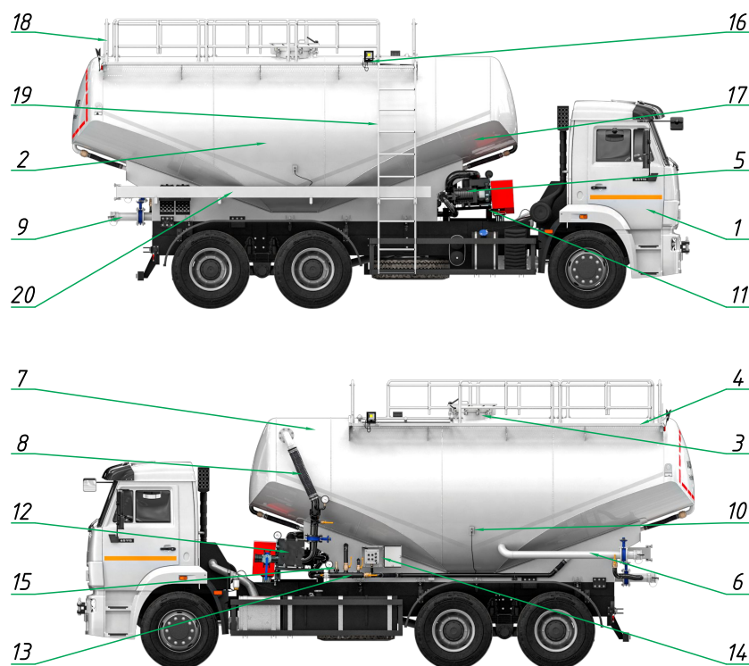
Figure 3 - ACV-17R1-05 Cement bulk truck.
