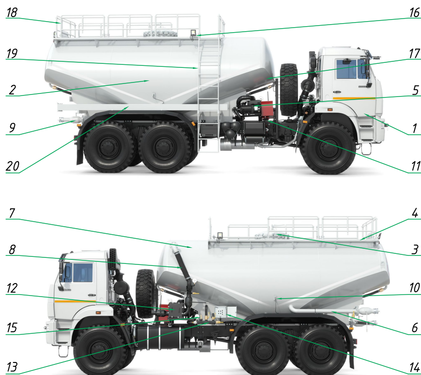
Figure 3 - ACV-17R1-01 Cement bulk truck.
